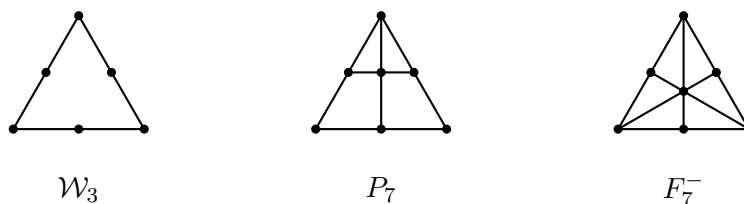
FIGURE 3. \mathcal{W}_3 , P_7 , and F_7^- .
